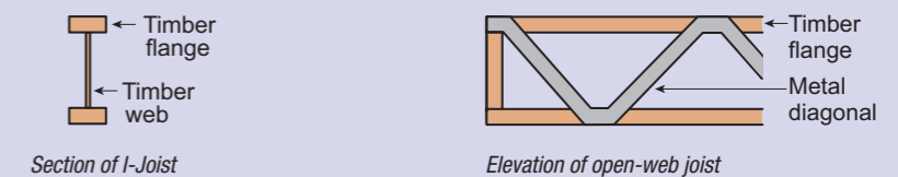
Section of I-Joist
