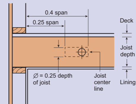
Safe drilling of joists
