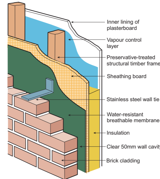
External wall and brick
