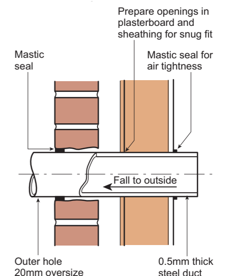
Fit the steel duct, making sure that it slopes downwards towards the outside
